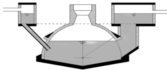
biogas plant
