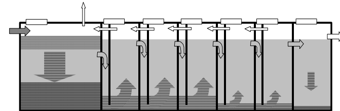
anaerobic baffled reactor
