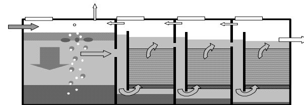
anaerobic filter
