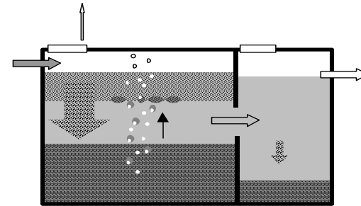
septic tank
