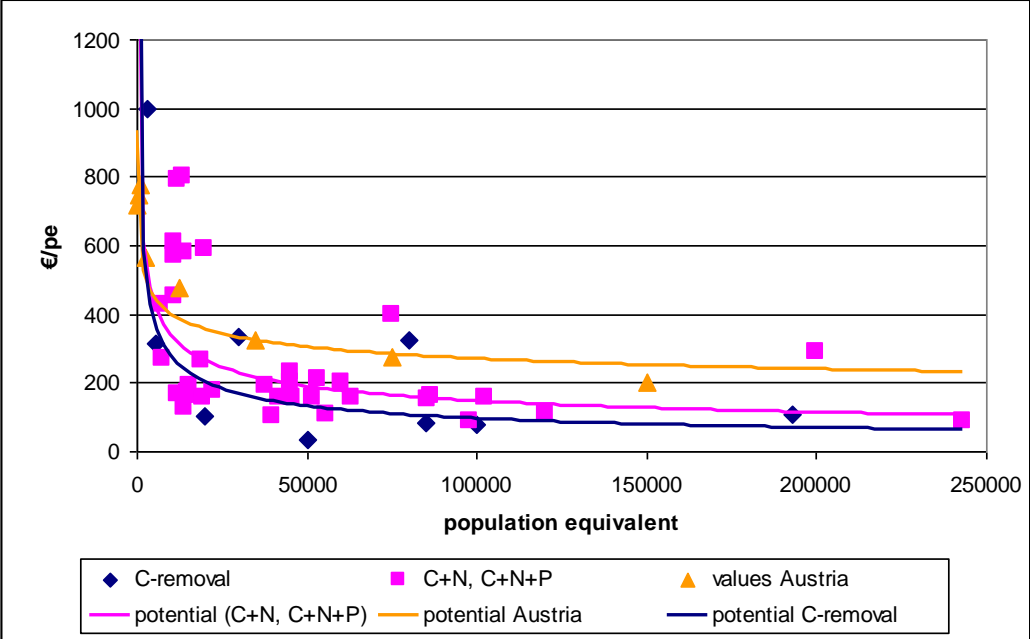
Figure 22: Investment costs for CND- and CNDP-plants in Danubian countries based on the Dablas report and CNDP-plants in Austria
