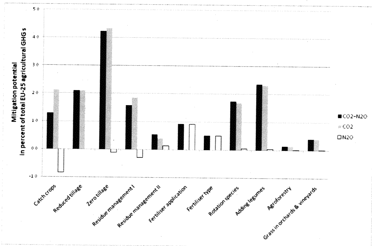
Figure 1 Mitigation potential of selected PICCMAT practices (MITERRA)
