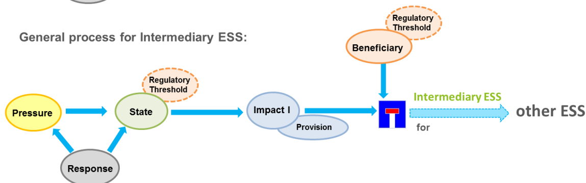
Figure 6. General scheme for Final ESS and Intermediary ESS for application of the DPSIR approach (P=Pressure, R=Response, S=State, I1=Impact I, I2=Impact II, B=Beneficiary, RT=Regulatory threshold)
