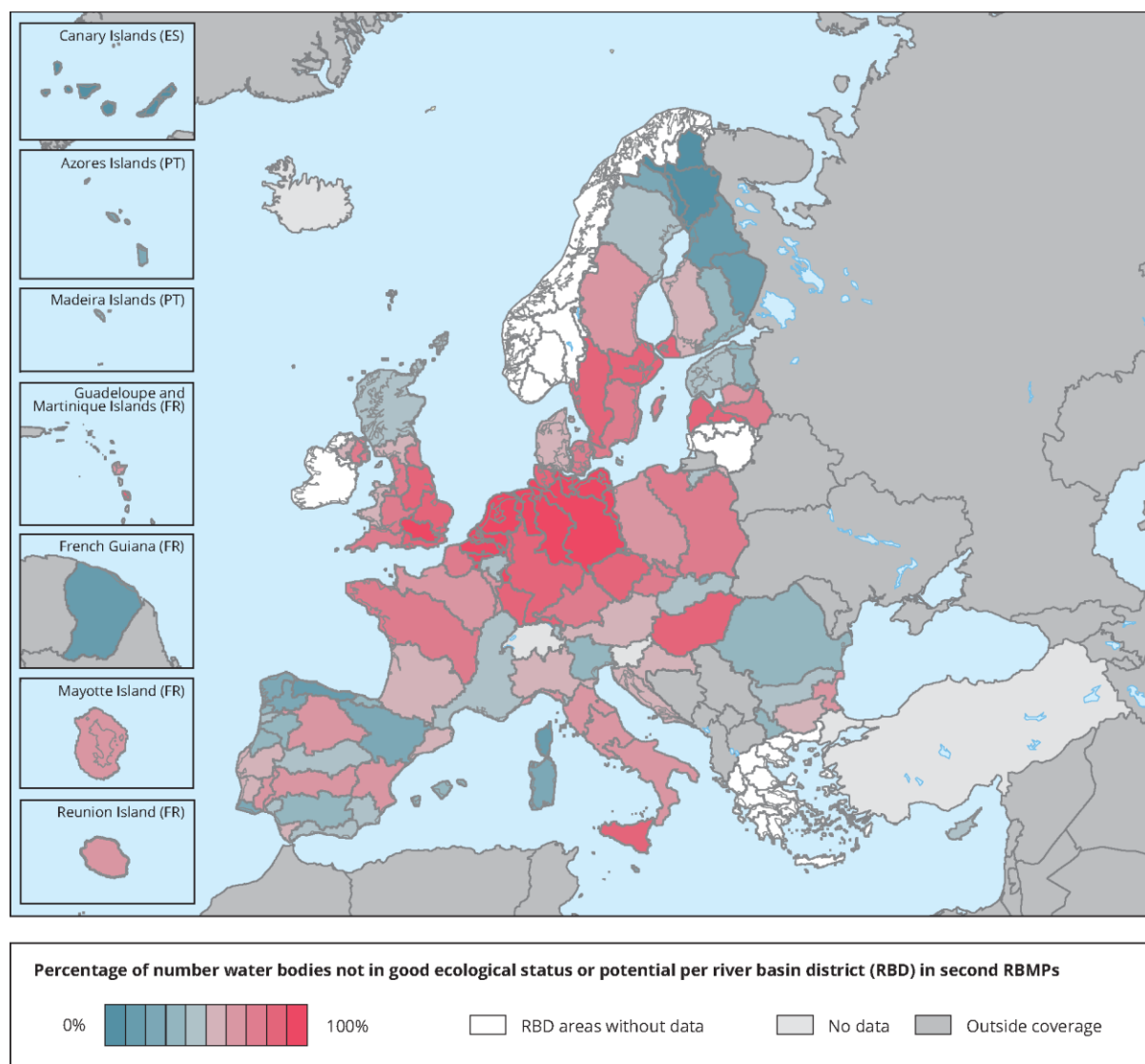
Figure 4-2 The percentage of waterbodies not in good ecological status or potential in Europe
